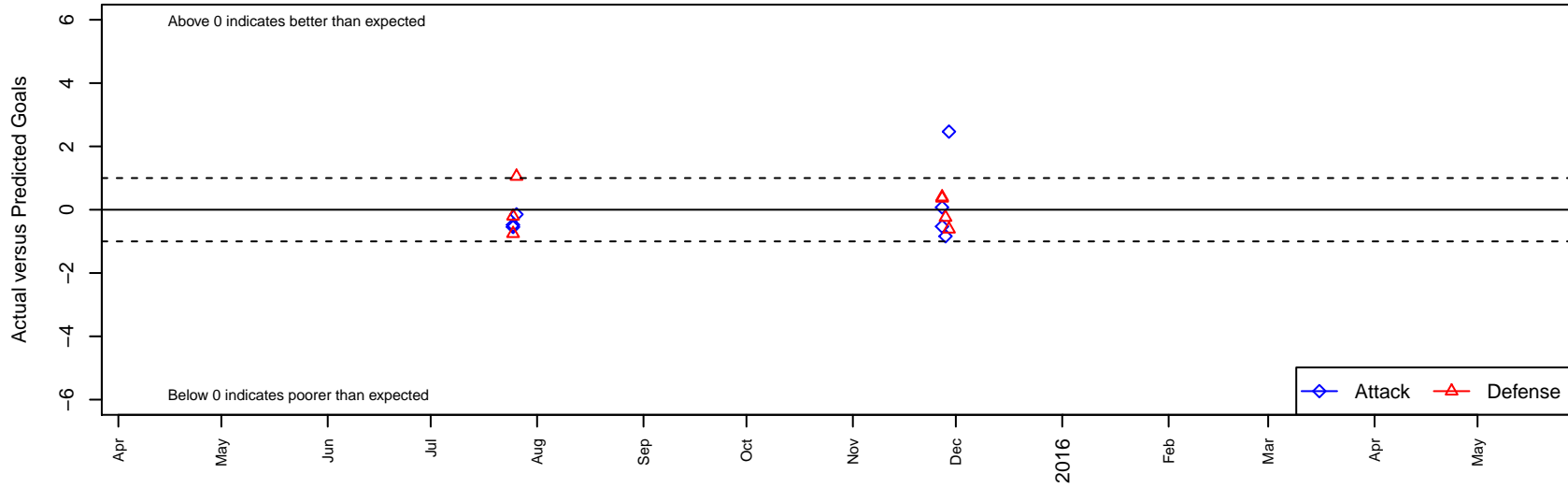
Placer United 99 Gold G98 Dots are actual minus expected GF (blue circles) and GA (red triangles). Blue line is smoothed change in attack strength. Red is smoothed change in defense strength.
